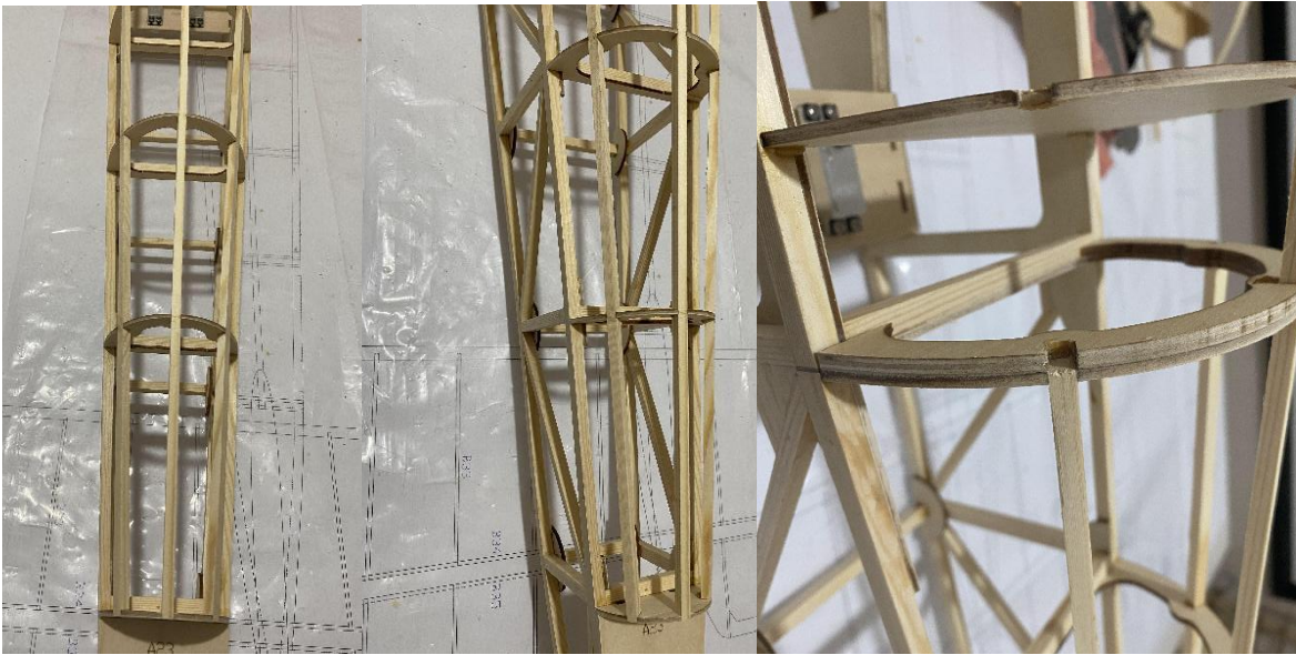
11) Glue the 1mm plywood fuselage cover.
