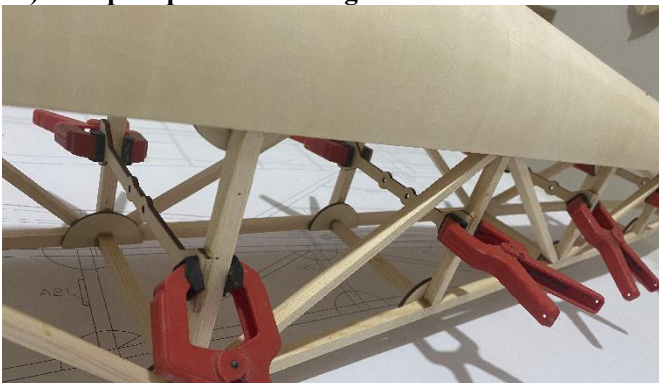
13) Glue scabbards, taking care to maintain the verticality of the scabbards.
